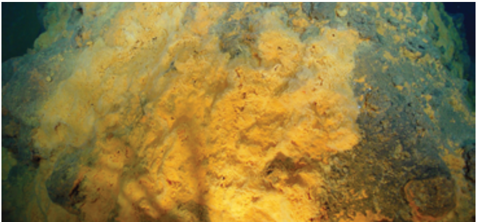
Bacteria grows near hydrothermal vents.
