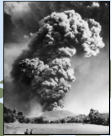
Paricutin volcano in Mexico
